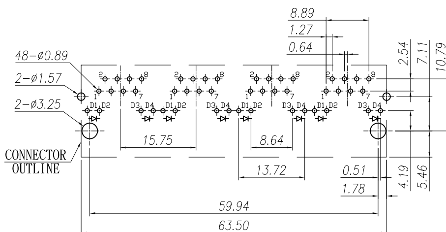
SUGGESTED PCB LAYOUT
