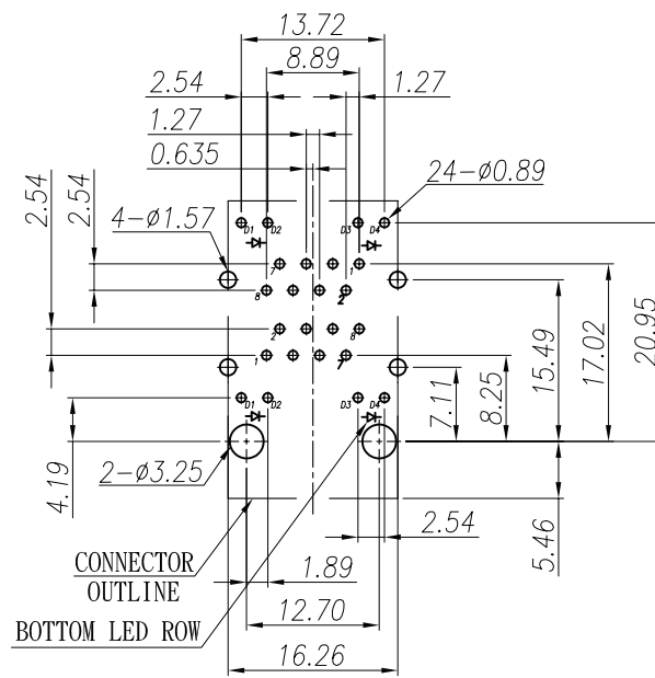
SUGGESTED PCB LAYOUT
