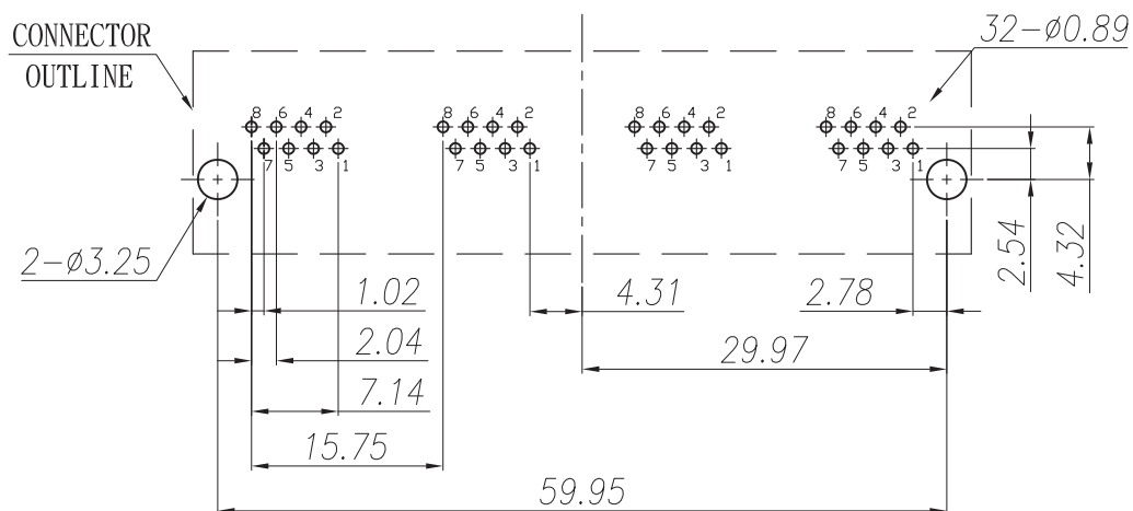
SUGGESTED PCB LAYOUT TOP VIEW DIMENSIONAL TOLERANCE: .XX \pm 0.08
