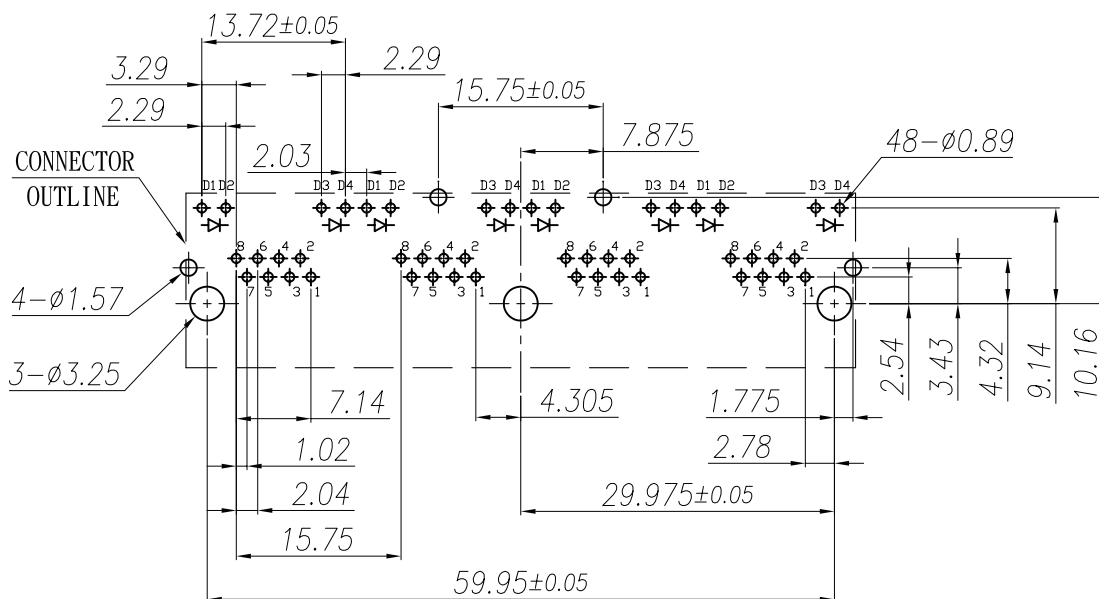
SUGGESTED PCB LAYOUT TOP VIEW
