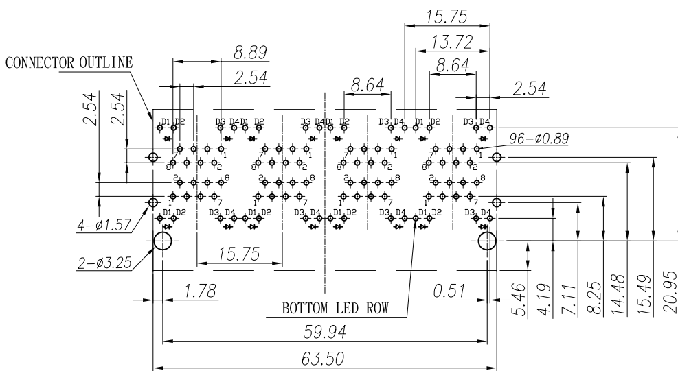
SUGGESTED PCB LAYOUT
